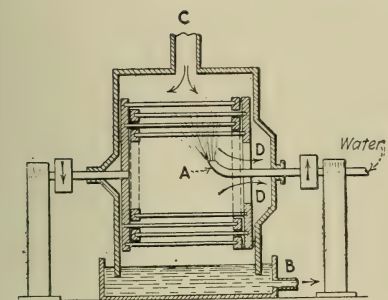
FIG. 68.—Schwarz-Bayer Disintegrator.
